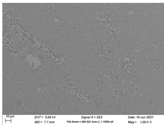
Image: Cross sectional SEM image of arc melted \text{ZrB}_2 - 58.5mol%SiC
