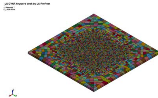
Image: Two-layer finite element model with stochastic material properties applied. Model elements were grouped in the through-thickness direction for the stochastic distribution of the material properties.
